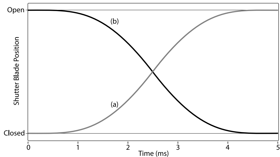
Figure 1.2: Shutter blade trajectory during a transition. Curve (a) illustrates the position of the shutter blade as it moves from the closed to the open position, and curve (b) illustrates the closing trajectory.
