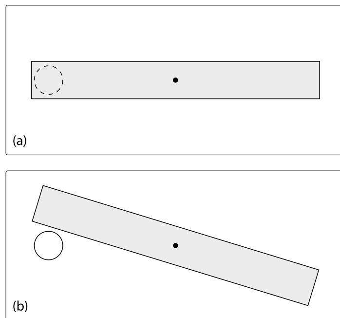
Figure 1.1: Mechanical action of the SR475 shutter head. Part (a) illustrates the shutter head in the closed position, where the shutter blade blocks the aperture. Part (b) shows the shutter head in the open position, where the shutter blade is clear of the aperture.
