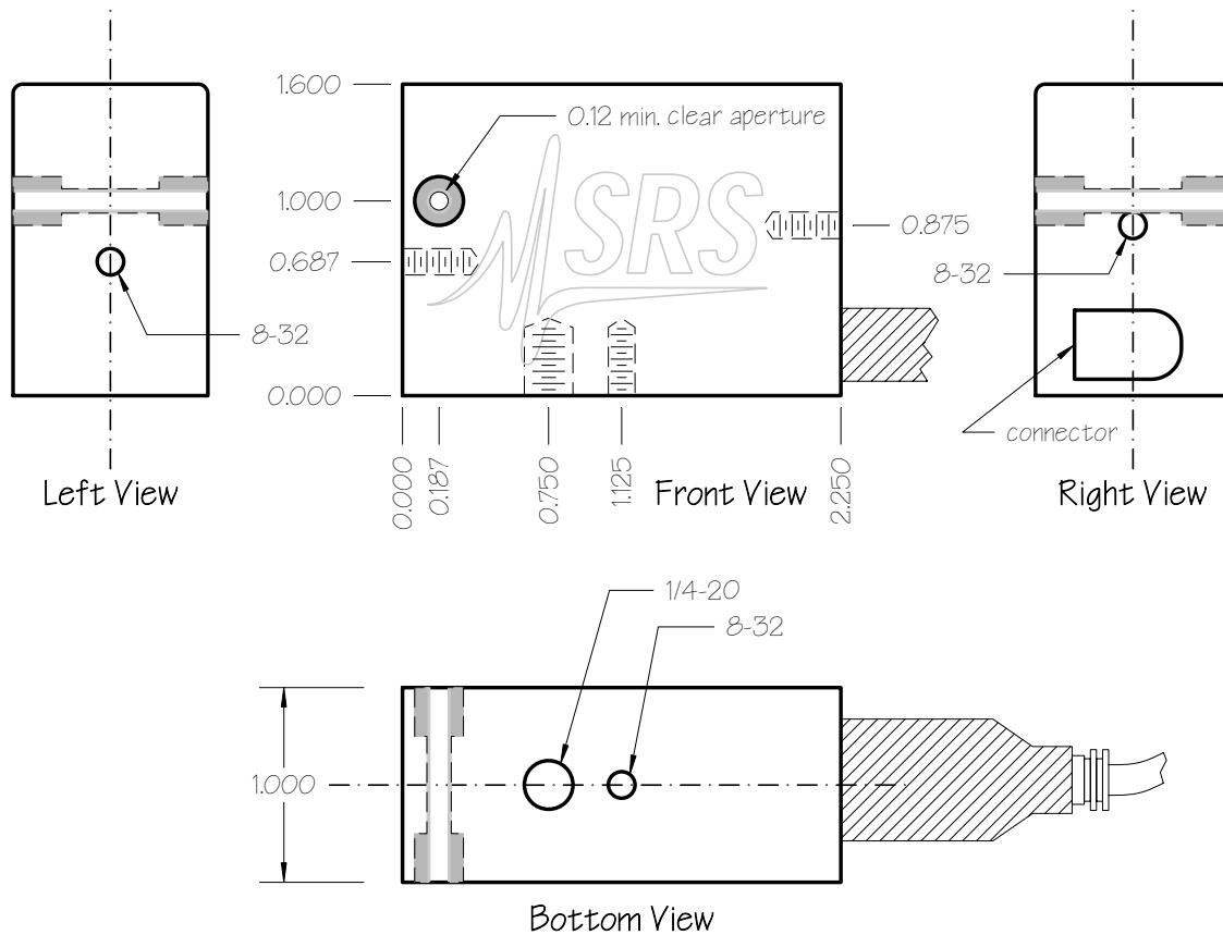
Figure 1.3: Physical dimensions and mounting of the SR475.
